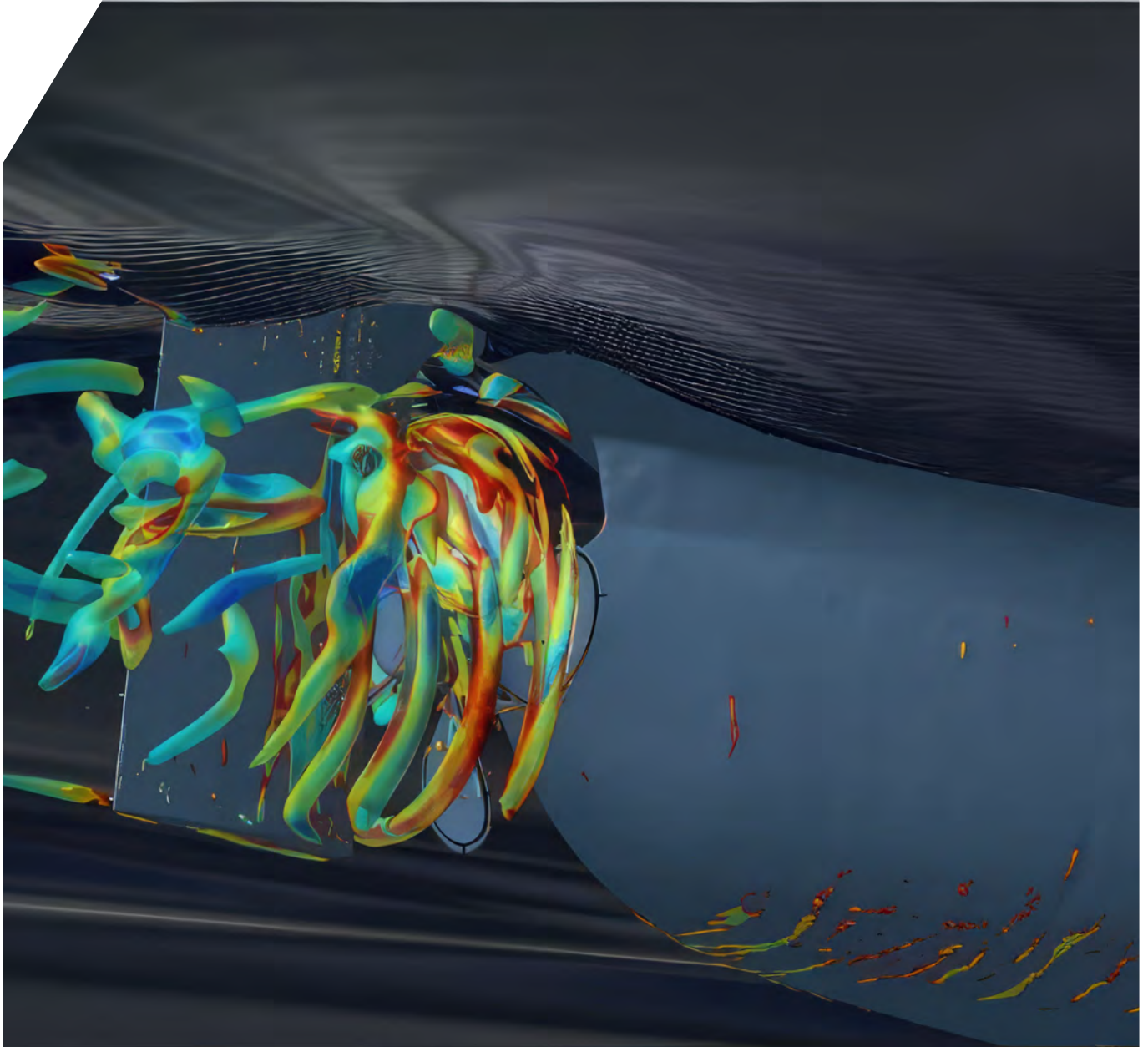
Hull-propulsor interaction
